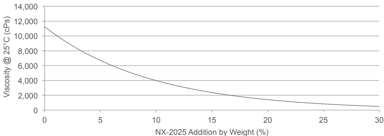
NX-2025 DILUTION CURVE WITH LIQUID EPOXY RESIN (EEW=190)
