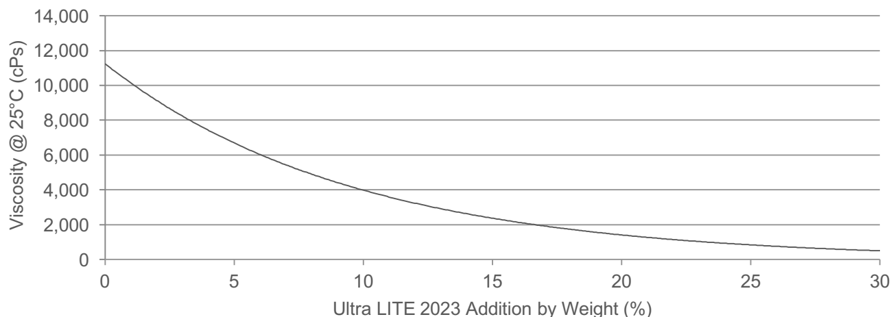
Ultra LITE 2023 DILUTION CURVE WITH LIQUID EPOXY RESIN (EEW=190)
